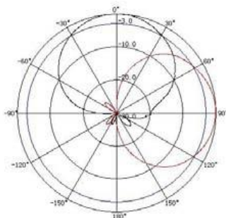
820 to 960MHz
